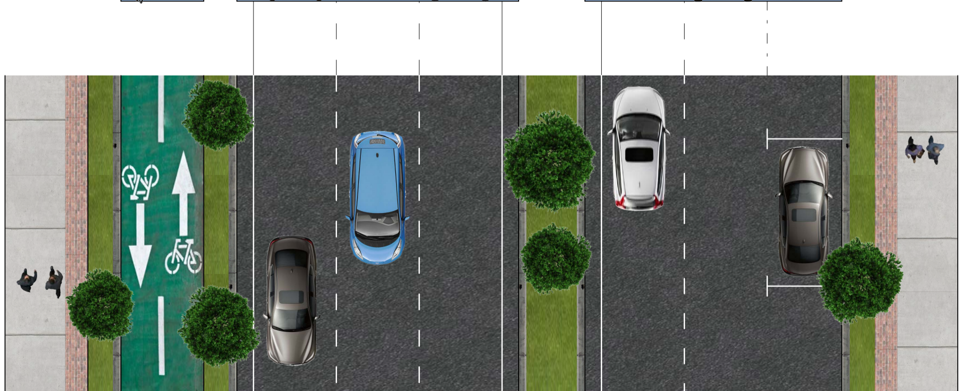
10' Sidewalk 4' 10' Cycletrack 4.5'-2' 11' Lane 11' Lane 11' Lane 2' 8' 2' 11' Lane 11' Lane 9' Parking Lane 4' 10' Sidewalk 120.5' (Varies at Median) Proposed Rt. 34 R.O.W.
